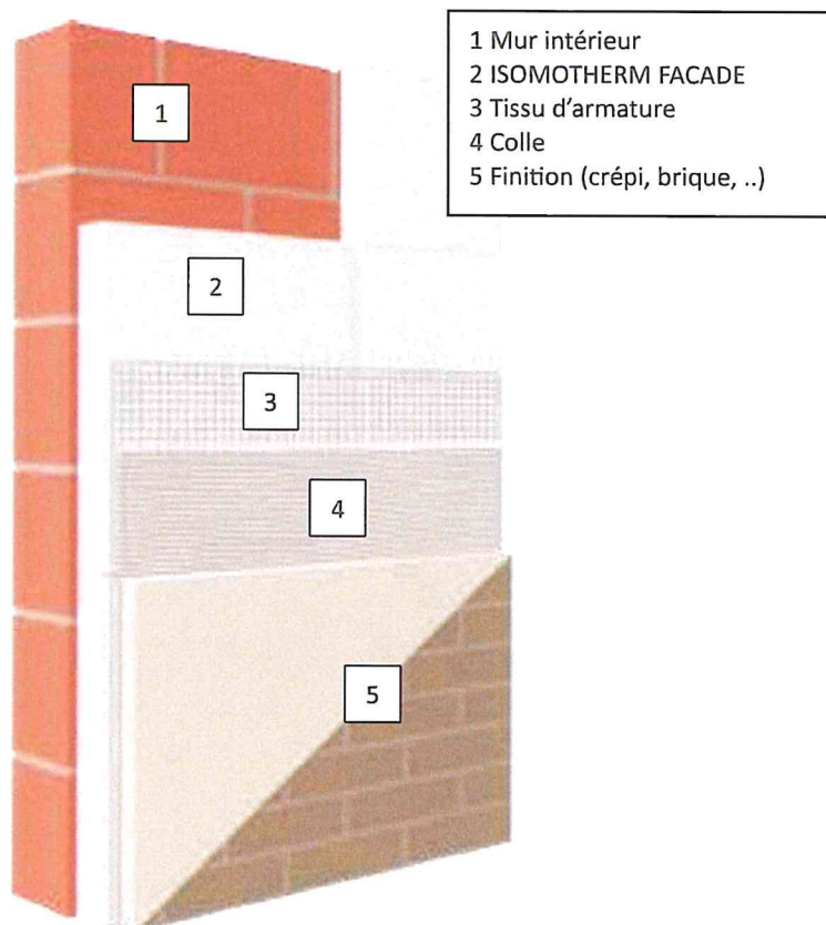
Figure 1: Utilisation de ISOMOTHERM FACADE
