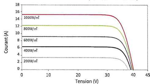
Courbe Courant-Tension (54HL4M-BDV 505W)
